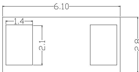
1-4 Soldering patterns 推荐焊盘
